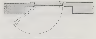
B SOLUTION: THIN SECTION OF WALL ADJACENT TO DOOR
